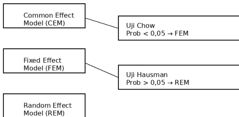
Gambar 1. Penentuan Model Regresi Data Panel
